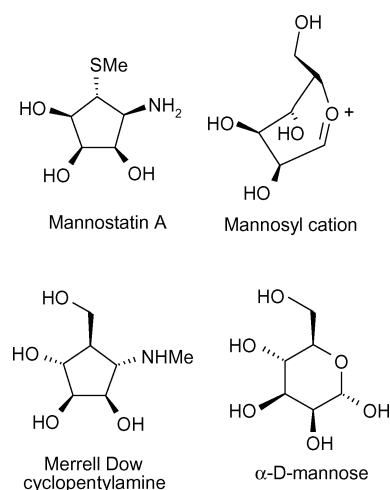
Fig. 2 Aminocyclopentanols as glycosidase inhibitors.
