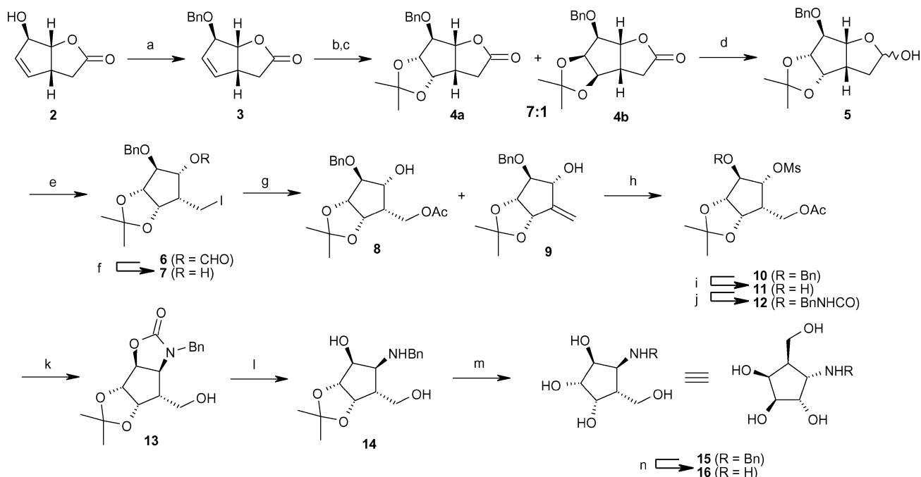
Scheme 1 Synthesis of aminocyclopentanols 15 and 16 . Reagents and conditions : a) \text{BnOCNCCl}_3 , dioxane, triflic acid, 0 °C, 10 min (81%); b) \text{OsO}_4(\text{s}) , NMO, \text{CH}_2\text{Cl}_2 , 25 °C, overnight; c) acetone, 2,2-dimethoxypropane, \text{H}_2\text{SO}_4 , 25 °C, 30 min (71% 4a ); d) DIBAL-H, \text{CH}_2\text{Cl}_2 , -78 °C, 1.5 h (88%); e) DIB, \text{I}_2 , cyclohexane, 250 W, 25 °C, 40 min; f) \text{Na}_2\text{CO}_3 , MeOH, \text{H}_2\text{O} , 25 °C, 2.5 h (61%); g) CsOAc, DMF, 65 °C, overnight (61% 8 , 17% 9 ); h) MsCl, DMAP, pyridine, \text{CH}_2\text{Cl}_2 , 25 °C, overnight (87%); i) Pd/C (5%), MeOH, EtOAc, 25 °C, overnight (90%); j) benzylisocyanate, \text{Et}_3\text{N} , \text{CH}_2\text{Cl}_2 , 25 °C, overnight (96%); k) KOtBu, THF, 25 °C, 35 min, then \text{H}_2\text{O} (72%); l) NaOH (2 M), ethanol, 65 °C, 2 h; m) HCl, \text{H}_2\text{O} , 60 °C, 5 h (65%); n) Pd/C (10%), EtOH, 25 °C, overnight (quant).
